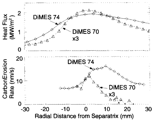
Fig. 5. (a) Radial profiles of heat flux and (b) net carbon erosion for DiMES 70 and DiMES 74.
