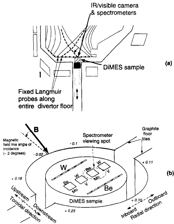
Fig. 1. (a) Poloidal cross-section of DiMES exposure. Sample is kept in private flux region until OSP is swept onto probe (dashed flux lines). (b) DiMES sample, metallic films and surrounding graphite tile geometry. Numbers indicate relative height of tiles to standard DiMES surface in mm. The gap between the sample and tiles is exaggerated for viewing clarity.
