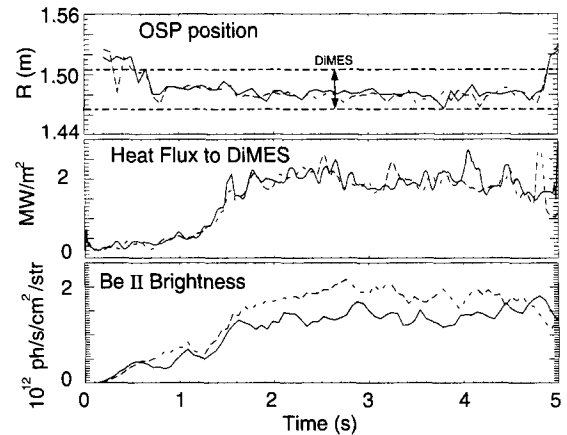
Fig. 2. Time traces of OSP position, heat flux and BeII ( 4673 \text{ \AA} ) brightness for first and third of the four DiMES 74 exposure discharges (solid line: #86987, dashed line: #86989).
