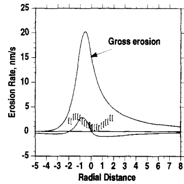
Fig. 7. Comparison of DiMES 70 carbon net erosion radial profile with REDEP calculations.
