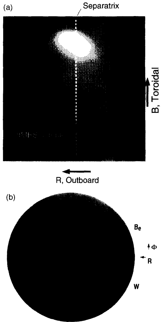
Fig. 4. (a) CII ( 5145 \text{ \AA} ) camera image of DiMES 74 exposure data line in separatrix position. The camera is saturated at the bright spot on the downstream tile. (b) Post exposure photograph of DiMES 74. Note the darkening of the usually shiny Be film and the arc tracks on the W film.
