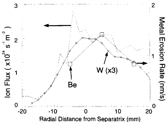
Fig. 6. Radial profiles of ion flux and beryllium and tungsten erosion rate for DiMES 74.
