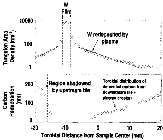
Fig. 3. (a) Toroidal distribution of tungsten areal concentration (from NRA) and (b) carbon redeposition (from RBS depth-marking) for DiMES 74. Regions with no carbon data are due to contaminating influence of metals on RBS depth-marking.
